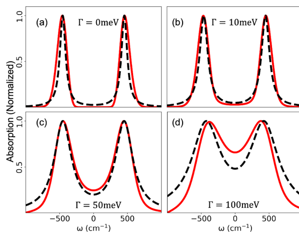
FIG. 4. A comparison between the \mathcal{L} -PLDM simulated linear spectra (red solid lines) with the analytic expression in Eq. (58) (black dotted lines), for the same model system shown in Fig. 3. The coupling strength g_c \approx 456 \text{ cm}^{-1} is fixed, whereas the cavity loss rate \Gamma varies. The analytic curve in Eq. (58) is obtained with peaks from the real part of Eq. (57) and Lorentzian broadening of the width given by the imaginary part of Eq. (57).
