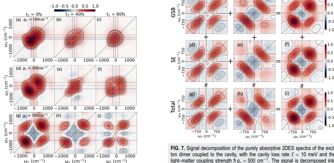
FIG. 6. Purely absorptive 2DES of the exciton dimer coupled to the cavity, with (a)–(c) g_c = 100 \text{ cm}^{-1} , (d)–(f) g_c = 200 \text{ cm}^{-1} , and (g)–(i) g_c = 500 \text{ cm}^{-1} for a lossless cavity ( \Gamma = 0 \text{ meV} ).
