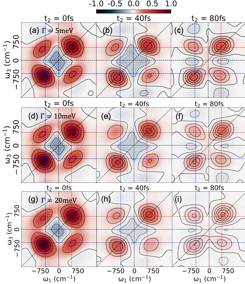
FIG. S5: Purely absorptive 2DES polariton spectra for the exciton dimer coupled to the cavity, with a fixed light-matter coupling strength \hbar g_c = 500 \text{ cm}^{-1} and various cavity loss rates.
