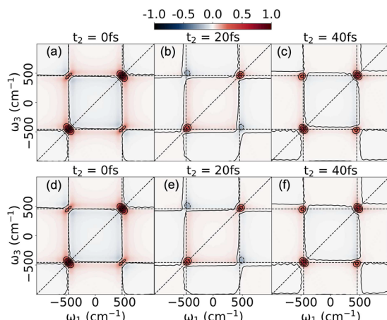
FIG. 10. 2DES spectra of an exciton monomer coupled to the cavity by setting exciton-phonon coupling to be zero \hat{H}_R + \hat{H}_{ex-R} = 0 . The light-matter coupling strength is \hbar g_c = 500 \text{ cm}^{-1} , and the cavity loss rate is \Gamma = 10 \text{ meV} . The spectra are calculated with (a)–(c) the original Lindblad approach [Eq. (19)] and (d)–(f) \mathcal{L} -PLDM dynamics [Eq. (25)].
