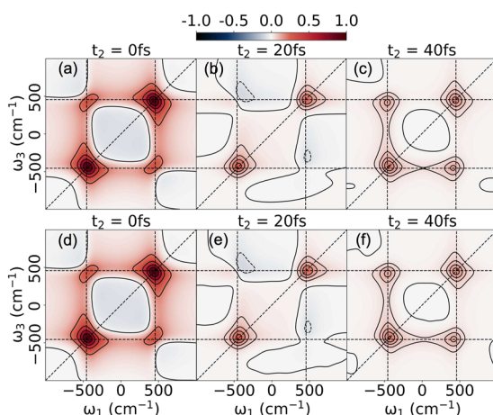
FIG. 11. 2DES spectra of a monomer coupled to the cavity. The same model parameters are used as in Fig. 10, except for the cavity loss rate \Gamma = 50 \text{ meV} . The spectra are calculated with (a)–(c) Lindblad and (d)–(f) \mathcal{L} -PLDM dynamics.
