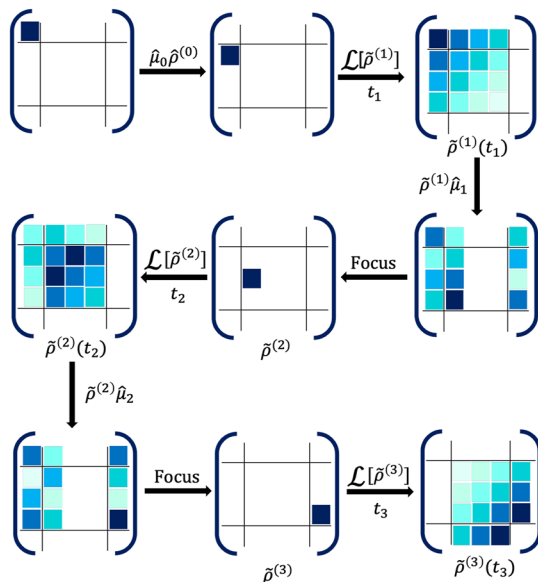
FIG. 2. Schematic illustration of the 2DES simulation algorithm, with one possible path [see Eq. (4) for all possible paths]. The color gradients imply the magnitude of the density matrix elements. \mathcal{L} indicates the overall time evolution by the \mathcal{L} -PLDM approach [see Eq. (29)], and \mu_i \tilde{\rho}^{(i)} (or \tilde{\rho}^{(i)} \mu_i ) indicate the dipole operator acting on the density matrix from the left-hand (right hand) side at time t = t_i .
