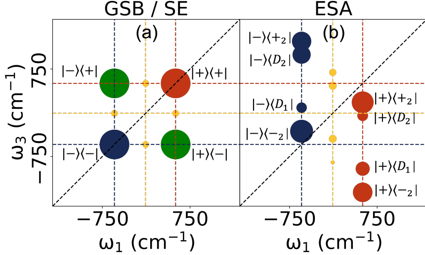
FIG. S3: Qualitative 2DES peak locations at t_2 = 0 fs for Fig. 8 of the main text. (a) GSB and SE peaks, (b) ESA peaks. The size of the circle corresponds to the expected signal intensities.
