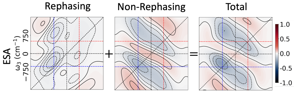
FIG. S4: The ESA contribution of the 2DES spectra for the exciton dimer coupled to the cavity.
