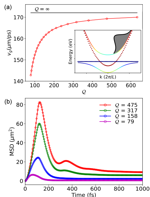
Figure 2. Group velocity dependence on quality factor for UP broadband excitation. (a) Polariton group velocity v_g vs cavity quality factor Q . The inset shows the energy bandwidth used for the initial excitation in the UP branch, optimizing the localization of the polariton wavepacket. Results are converged with 250 trajectories, validated against a set of runs with 1000 trajectories. (b) Time-dependent transient MSD with UP initial excitation for various Q .
