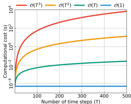
FIG. 2. Computational cost scaling as a function of the number of time steps ( T ) of each laser pulse delay at different levels of vectorization of Eq. (39). The red curve denotes the computational cost of serial computation for a single trajectory of three laser pulses. The yellow curve denotes the computational cost when one of the lasers is vectorized. The green curve is the case of vectorization along two laser pulses and the blue curve denotes vectorization along all the laser delays. Each curve involves propagating a wavefunction in the 2D excitation manifold of \approx 50 molecules with around 2500 total quantum states. The above-mentioned calculations were performed on NVIDIA Hopper H100 GPUs using pytorch 48–50 with device “meta.” Each of the curves above is averaged over 10^6 instances of Eq. (39) operations.
